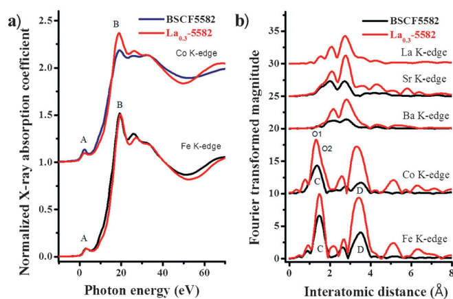
Figure 5. a) Normalized Fe and Co K-edge XANES spectra and b) radial distribution function for the all atomic EXAFS spectra for BSCF5582 and La 0.3 -5582. The Fe and Co XANES spectra have been plotted with respect to each absorption edge-energy (Fe = 7112 eV and Co = 7709 eV).
